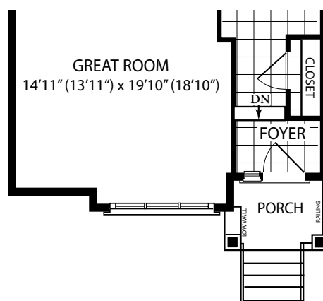
Main Level Elev E
