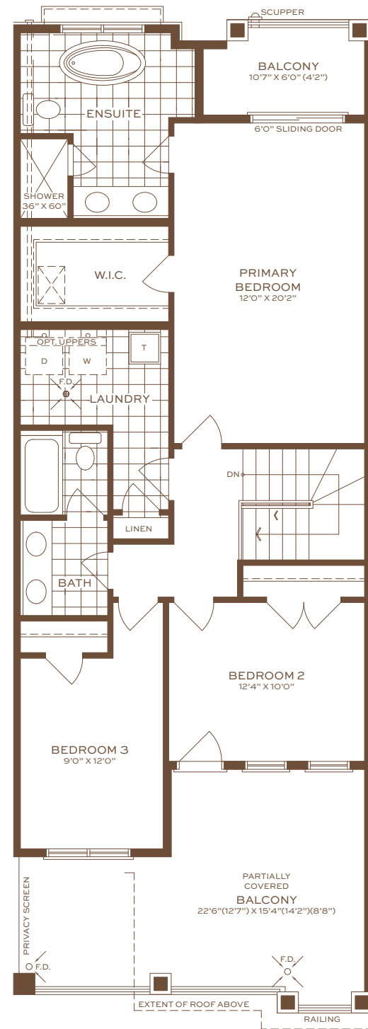
Second Floor Elevation A1 / A2
