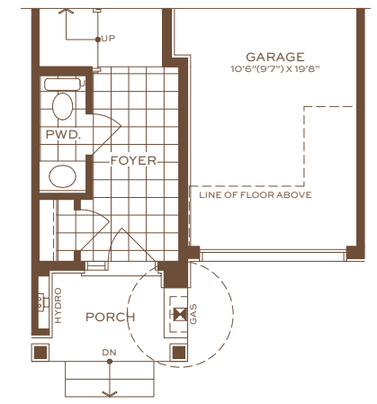
Partial Main Floor Elevation B
