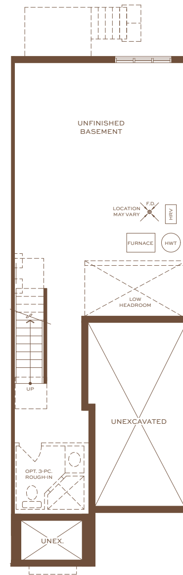
Basement Elevation A/A MOD./B
