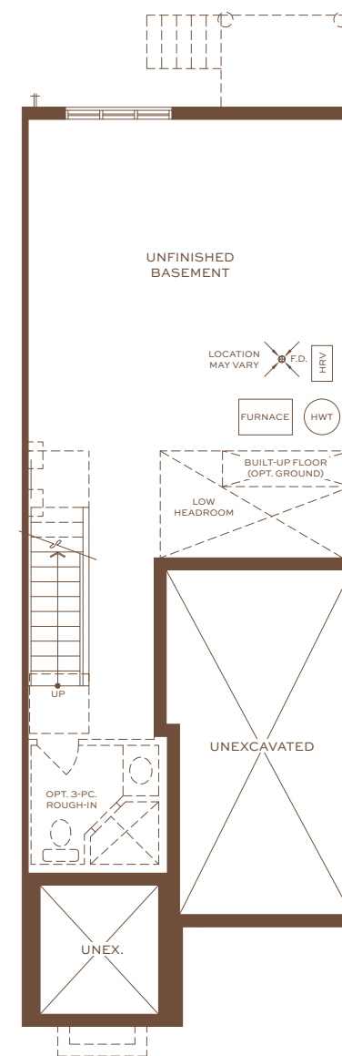
Basement Elevation A/A MOD./B
