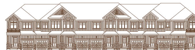
Front Elevation B (Building 5)
