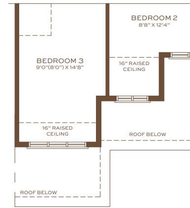
Partial Second Floor Elevation A
