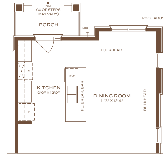
Partial Ground Floor Elevation B
