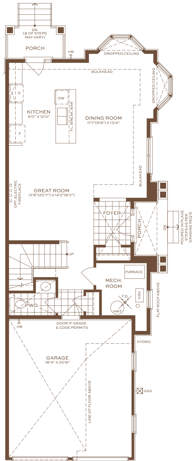
Main Floor Elevation A
